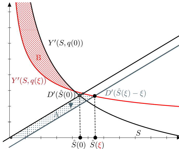
Figure 4: Competing welfare effects of type I geoengineering.
