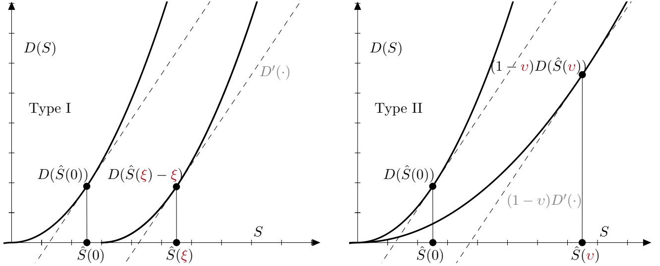
Figure 5: Environmental damage before and after type I (“carbon removal”) and type II (“climate adaptation” or “solar radiation management”) geoengineering. The left (right) panel depicts the increase in \hat{S} necessary to keep marginal damages constant with a type I (type II) technology.
