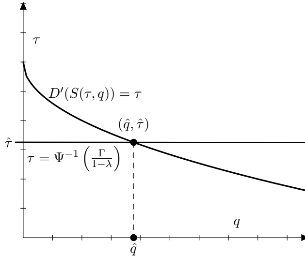
Figure 1: Unique interior equilibrium (\hat{\tau}, \hat{q}) .
