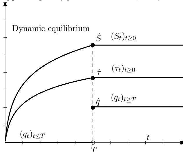
Figure 6: Time paths of the carbon stock (S_t)_{t \geq 0} , optimal taxes (\tau_t)_{t \geq 0} , and clean technology (q_t)_{t \geq 0} in the dynamic equilibrium.
