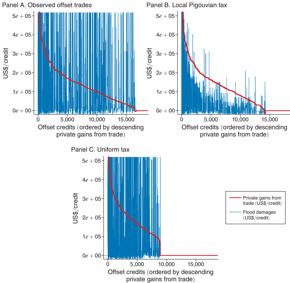
FIGURE 6. PIGOUVIAN REDESIGN
